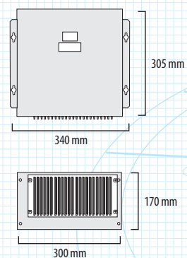
NDC-1417 Mass 6 kg
